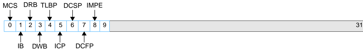
Figure 10-34. Machine Check Status Register (MCSR)
