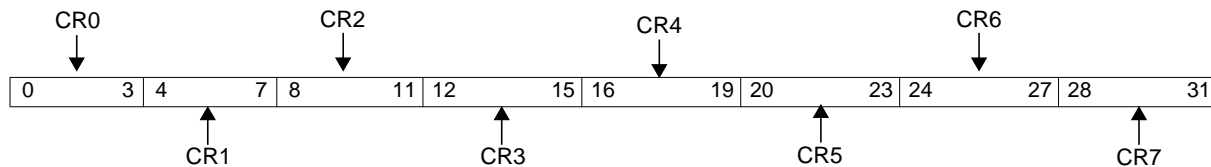
Figure 10-3. Condition Register (CR)
