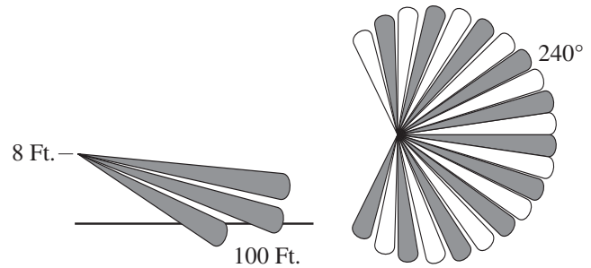
Figure 2 Coverage Angles
