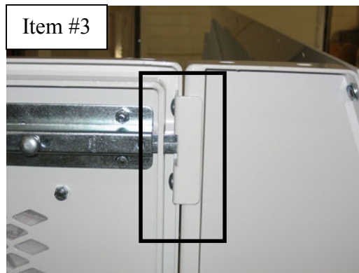
View of Emergency Exit Hatch support bracket assembled.
