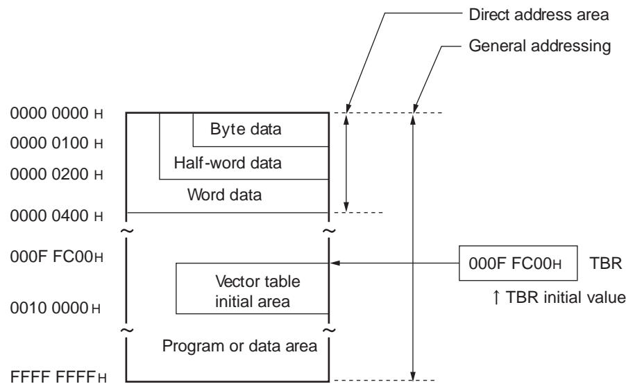
Figure 2.1-1 Address space
