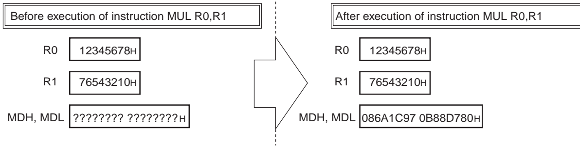
Figure 3.3-19 Example of Multiplication Operation using Multiplication/Division Register (MDH, MDL)
