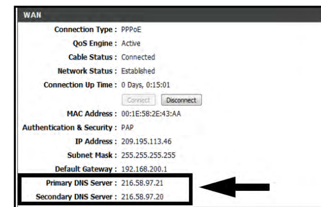
WAN Settings Example
