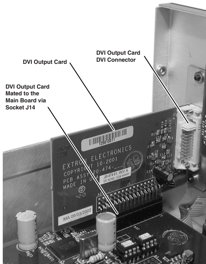
Figure 3 — Output DVI board installation
