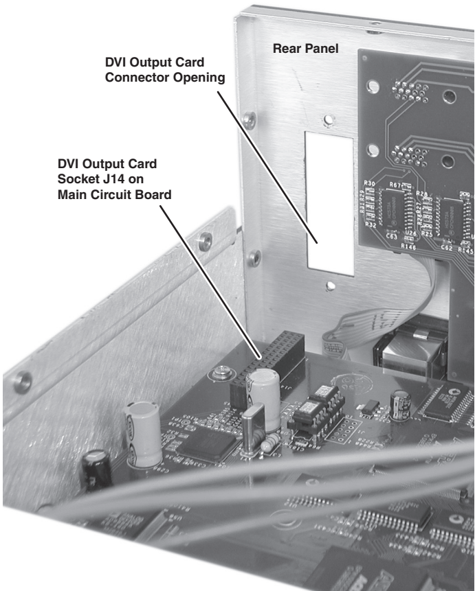
Figure 2 — DVI output card connector opening and socket J14
