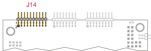
Figure 9. J14 Connector Layout
