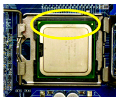
Fig. 3 Notice the small gold colored triangle located on the edge of the CPU socket. Align the indented corner of the CPU with the triangle and gently insert the CPU into position. (Grasping the CPU firmly between your thumb and forefinger, carefully place it into the socket in a straight and downwards motion. Avoid twisting or bending motions that might cause damage to the CPU during installation.)
