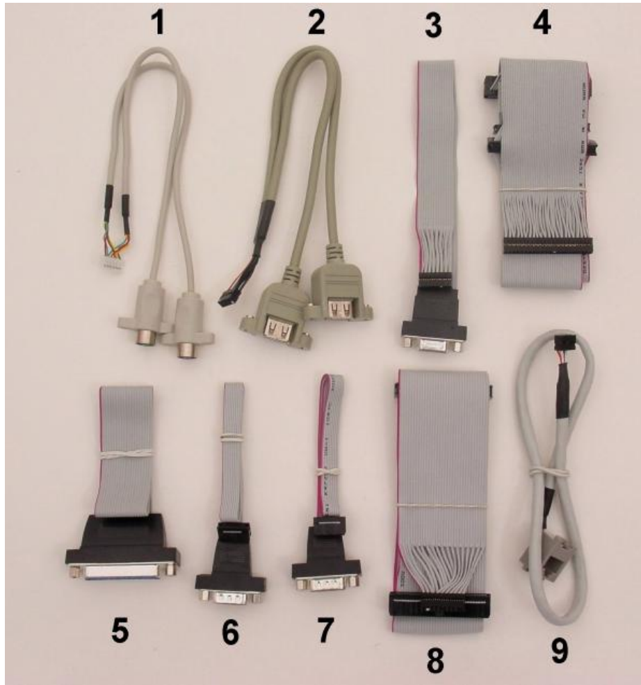
Figure 2. Morpheus Cable Kit
