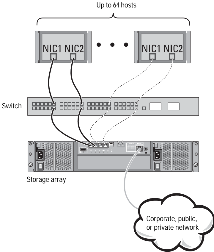
Figure 2-6. 64 Servers Connected to a Single Controller
