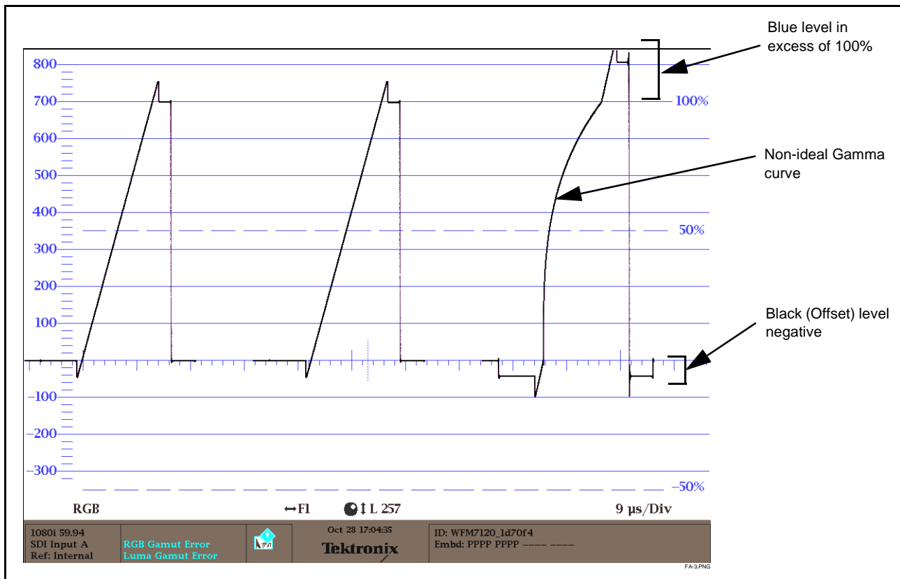
Figure 3-10 Uncorrected (Uncompensated) Monitor Waveform
