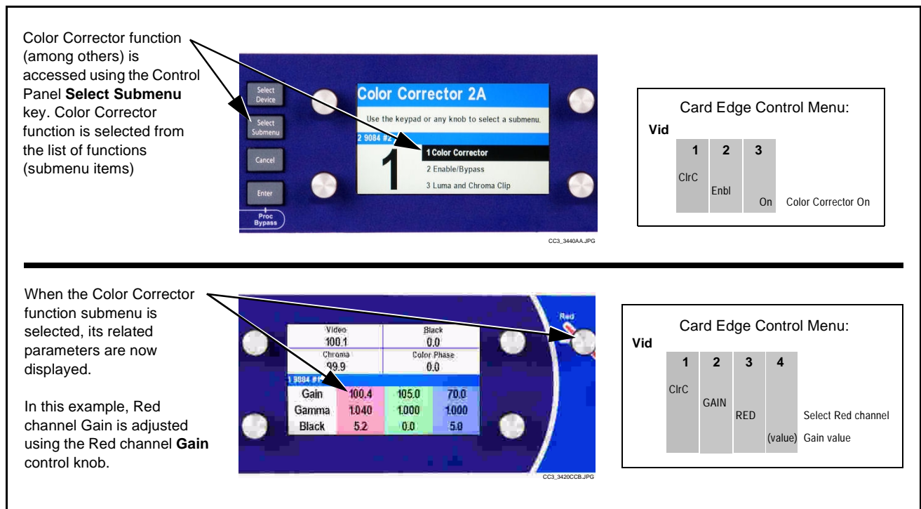
Figure 3-6 Control Panel Setup of Example Video Proc Function
