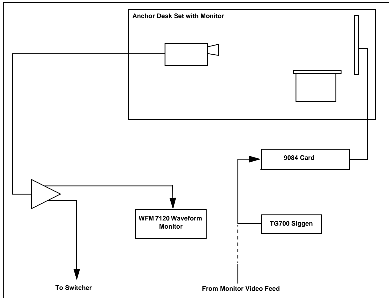
Figure 3-11 Example Setup Using Control Panel Color Corrector Function
