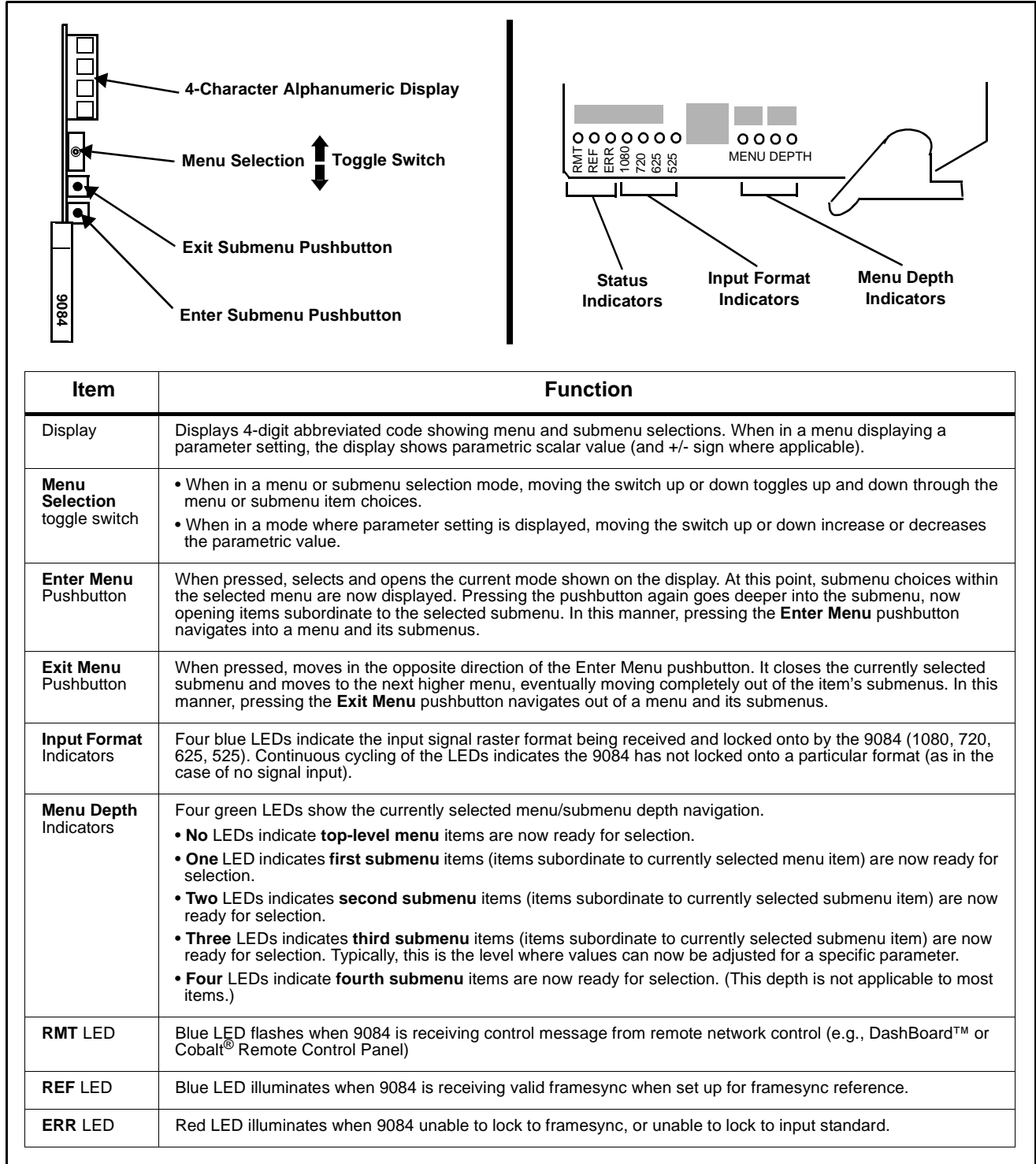
Figure 3-2 9084 Controls, Indicators, and Display
