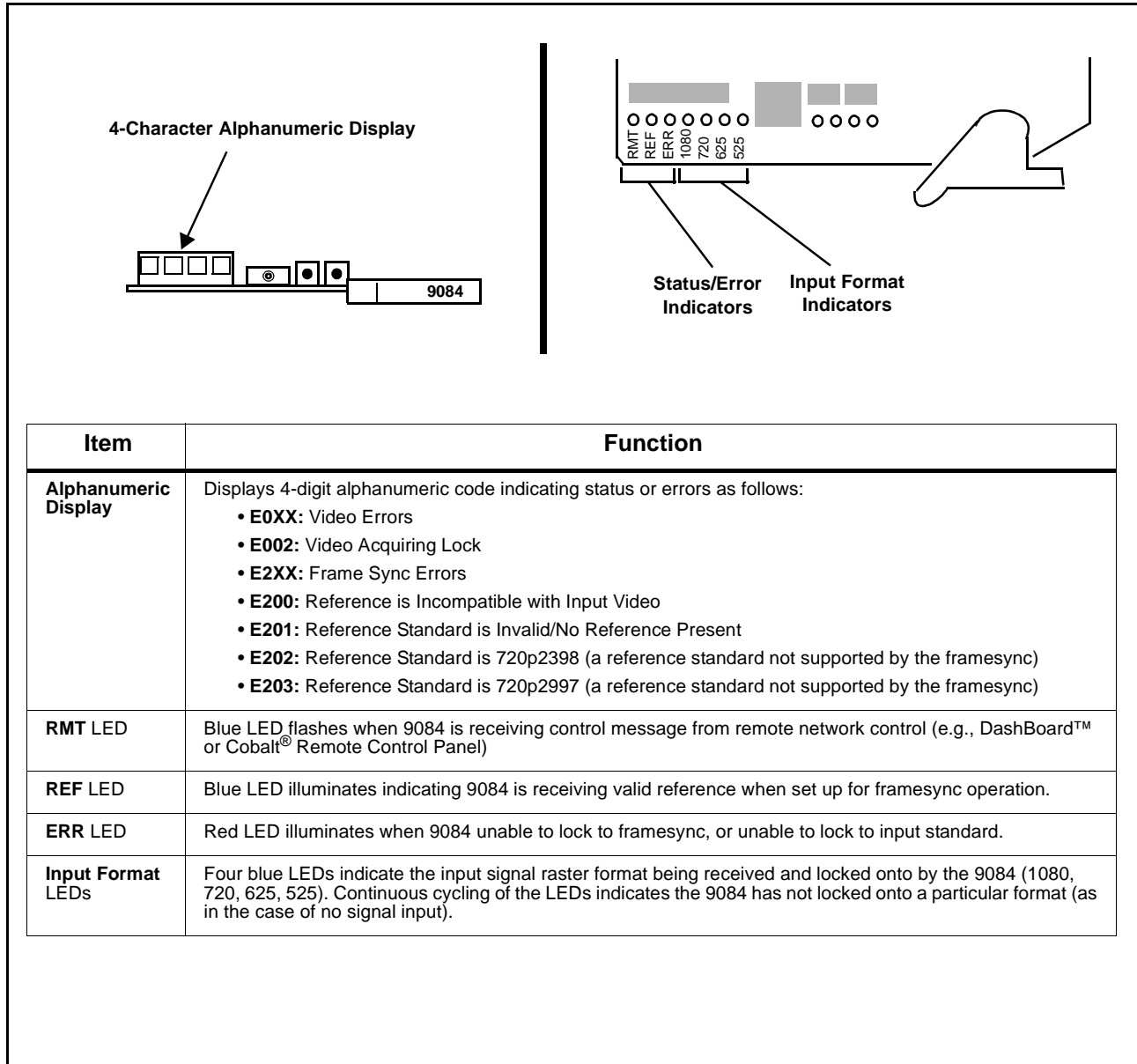
Figure 3-13 9084 Card Edge Status Indicators and Display
