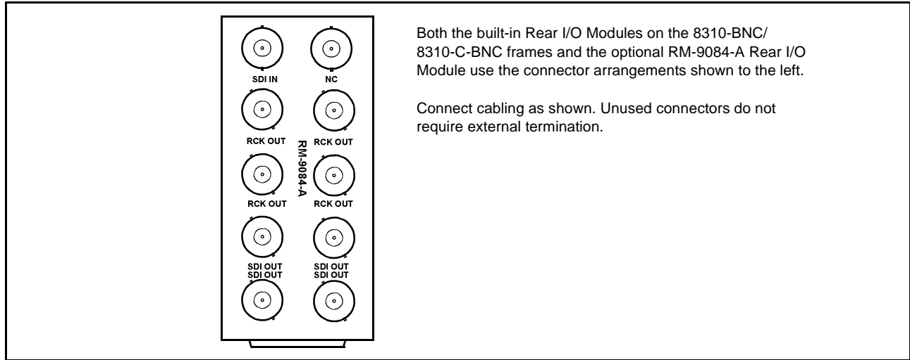
Figure 2-1 9084 Rear I/O Module Connections
