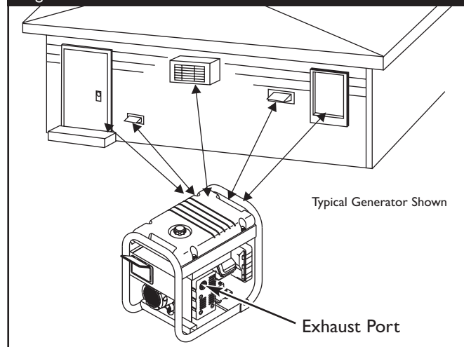
Figure 2 — Generator Clearance
