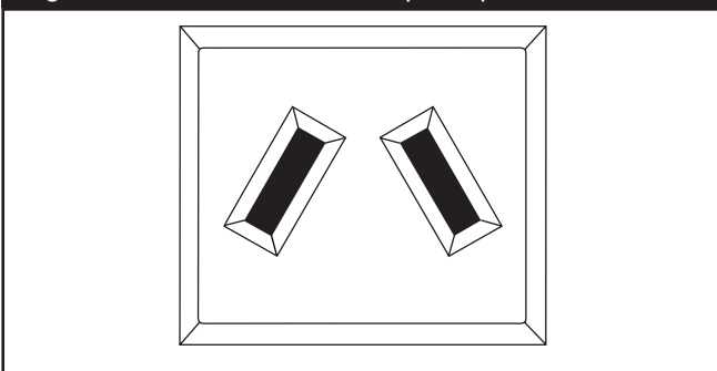
Figure 45 — 12 Voltios DC, 10 Amp Receptáculo
