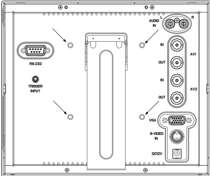
Figure 5.2 Location of mounting holes
