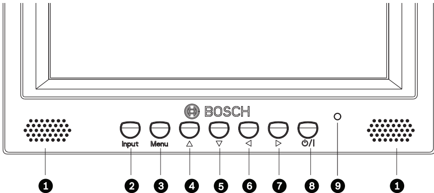
Figure 3.1 Front Panel
