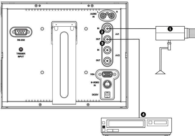
Figure 5.5 Single Monitor Configuration
