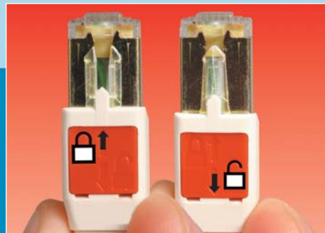
Simply push the boot forward to latch into the outlet. Then pull back to release. No thumbtabs to break.
