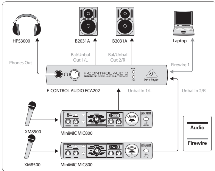
Fig. 4.3: The FCA202 as a laptop audio interface
