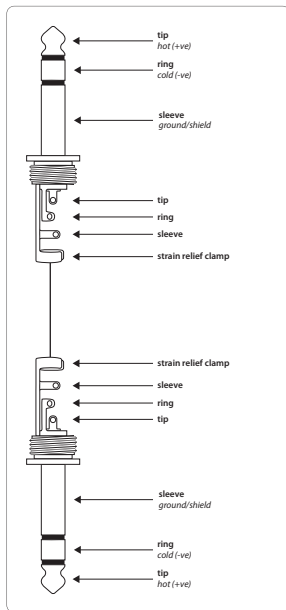
Fig. 5.2: Balanced jack cable with 1/4" TRS jack plugs
