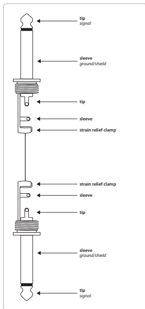
Fig. 5.1: Unbalanced jack cable with 1/4" TS jack plugs
