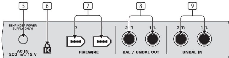
Fig. 3.2 back of the FCA202
