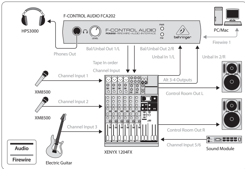
Fig. 4.2: Studio setup with the FCA202
