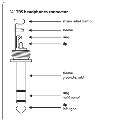
Fig. 5.3: Stereo jack plug for a set of headphones
