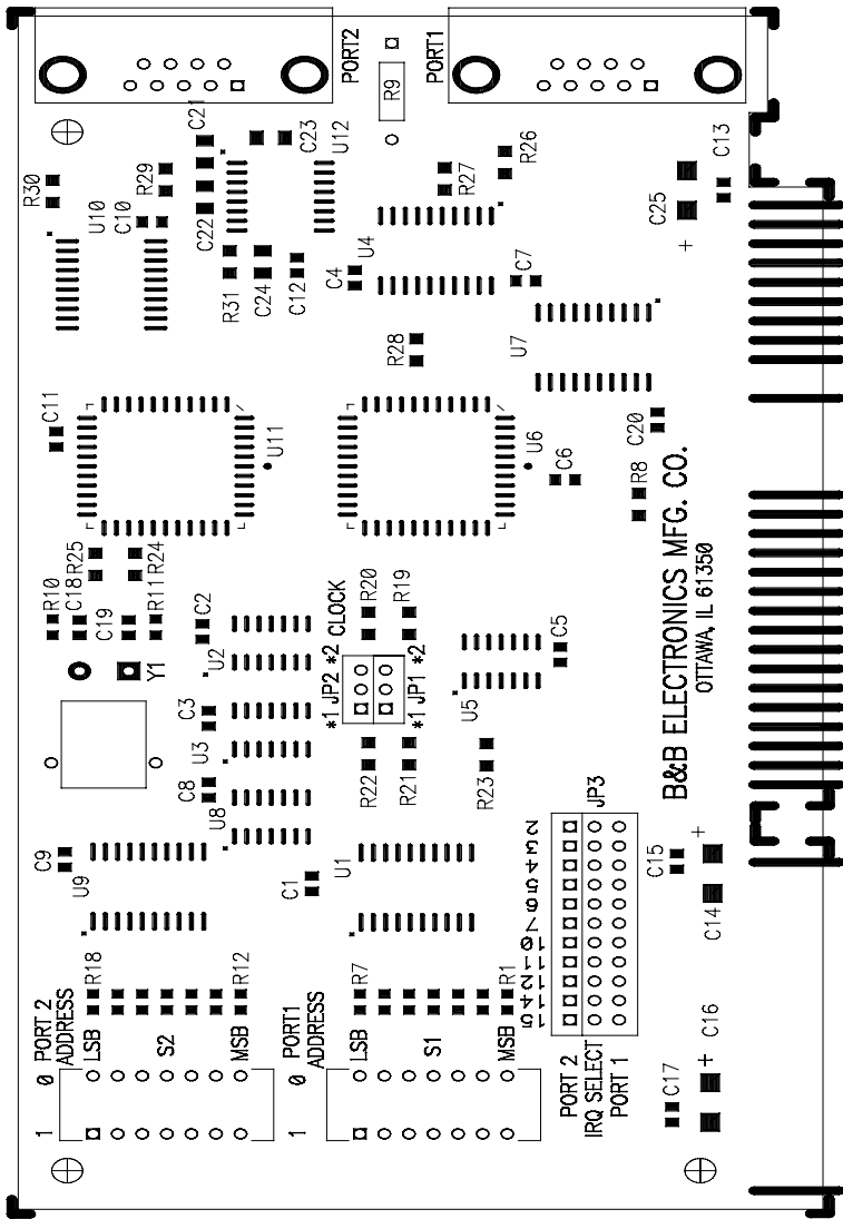
Figure 1. Silk Screen Plot of 232CC PCB
