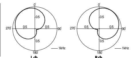
POLAR PATTERN
