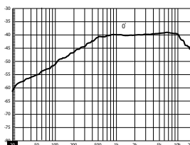
FREQUENCY RESPONSES
