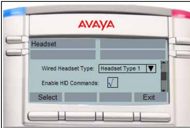
Figure 21: Headset screen
