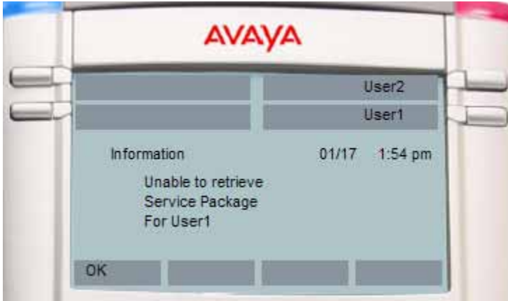
Figure 51: Per-account notifications
