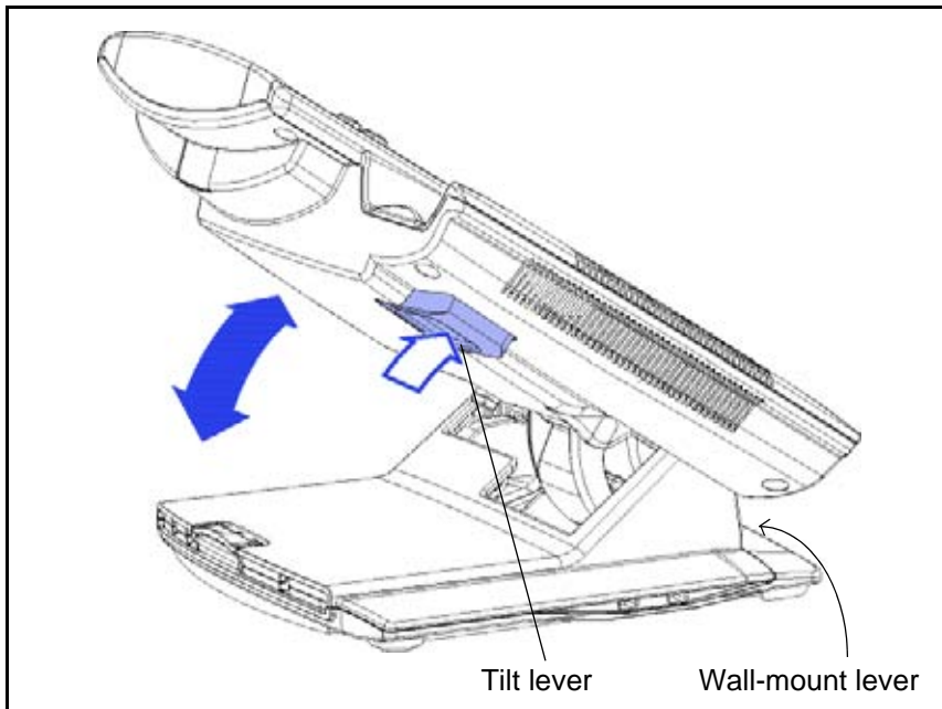
Figure 13: Rotate the IP Deskphone into the wall mount position
