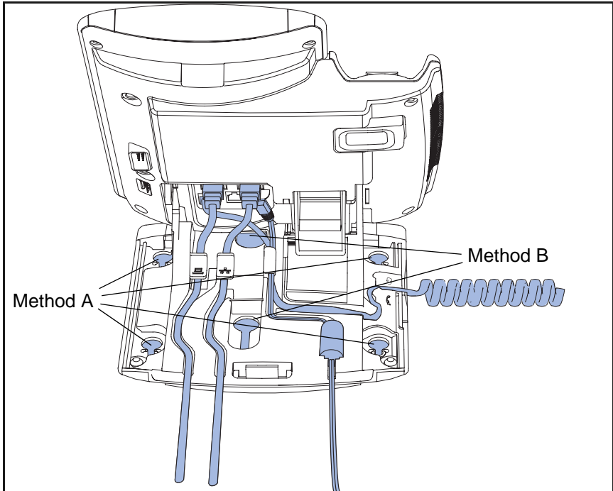
Figure 12: Cable routing tracks and mounting holes
