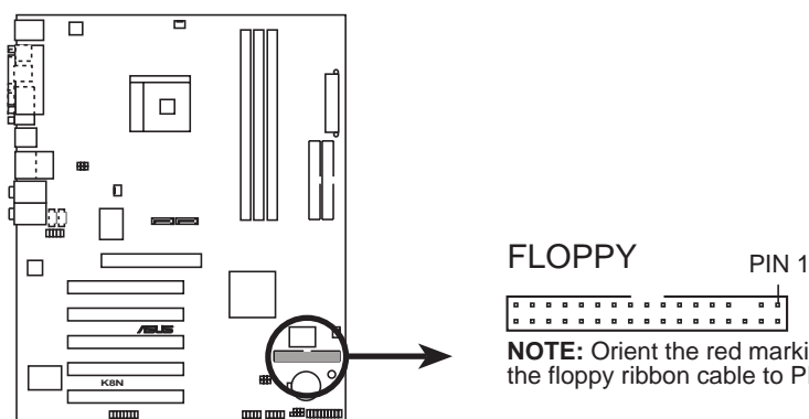
K8N Floppy disk drive connector
