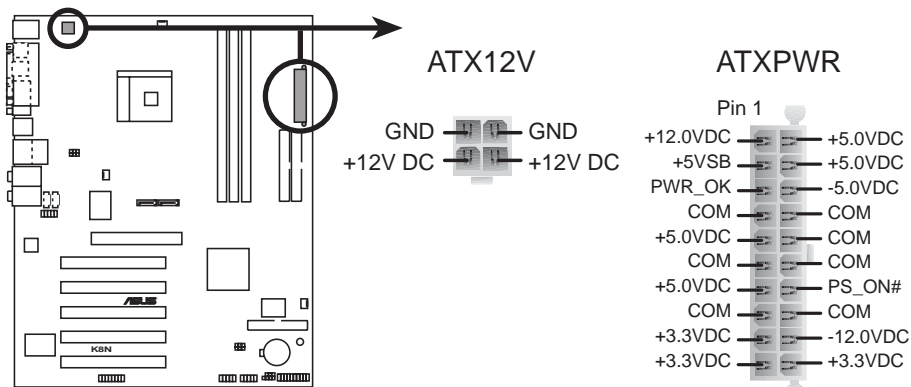
K8N ATX power connectors
