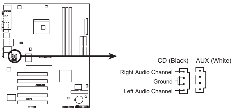
K8N Internal audio connectors
