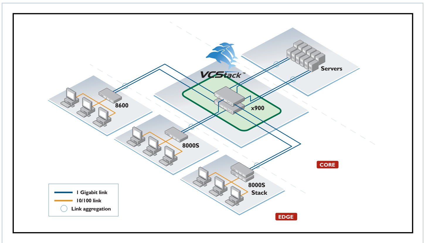
Diagram I: VCStack + Link Aggregation
