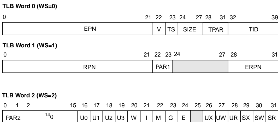
Figure 5-5. TLB Entry Word Definitions
