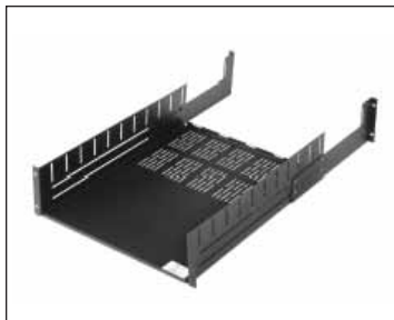
SH22-3 (with SHRSB3)
