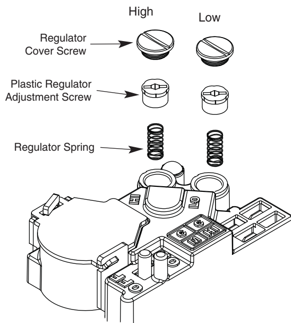
Figure 1. 36G/36J 2-Stage models
