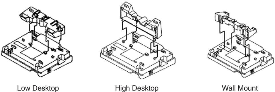
Figure 2-1 Footstand Mounting
