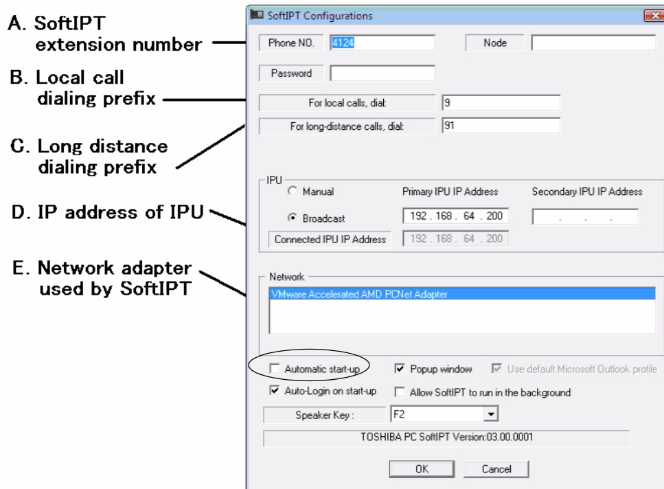
Figure 1 SoftIPT Configurations
