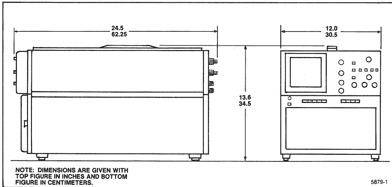
Figure 1-1. 7934 dimensional drawing.
