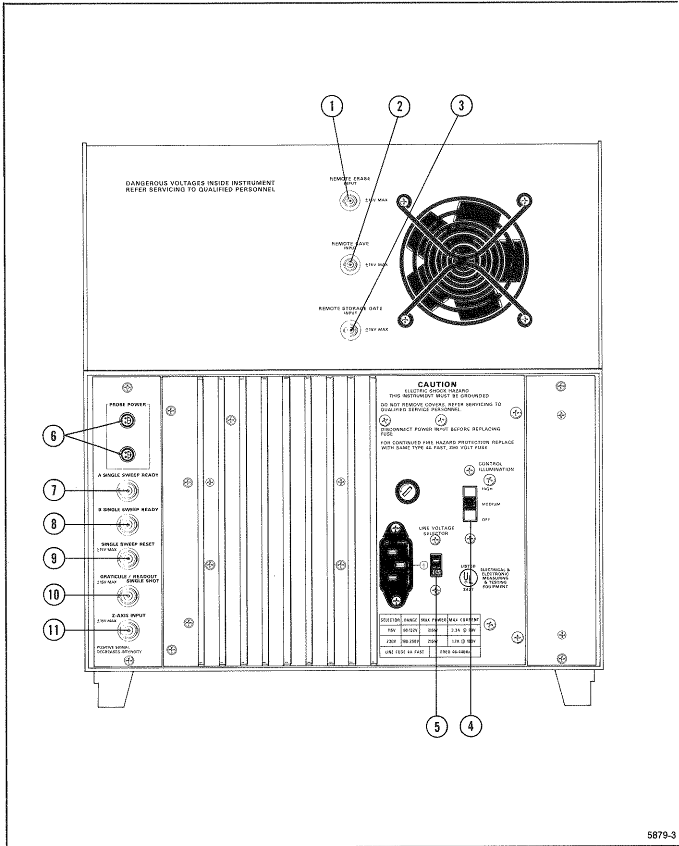
Fig. 2-2a. Rear-panel controls and connectors.
