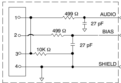
Fig. 1C (LEMO 4 PIN) MIC JACK BOARD
