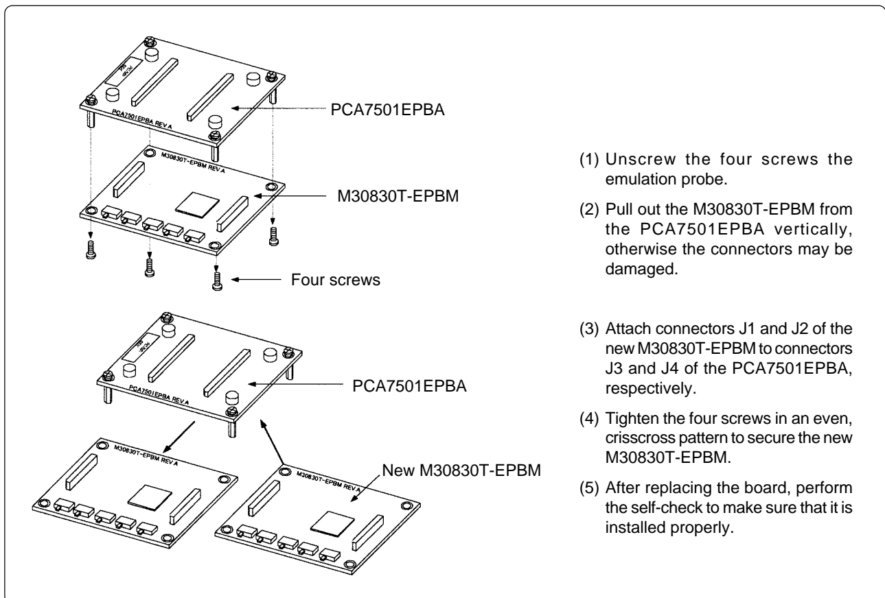
Figure 1 Replacing MCU boards
