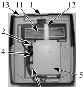
Inside slim base
