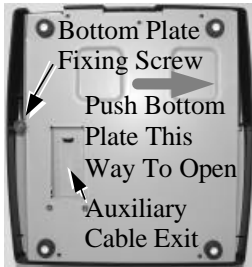
Slim base bottom
