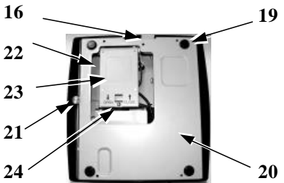
Universal Base 2.5" HDD
