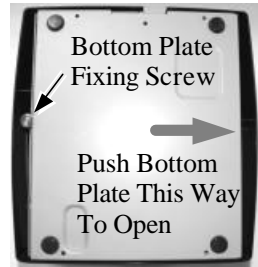
Universal base bottom
