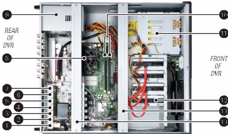
Figure 6. DX8100 Interior
