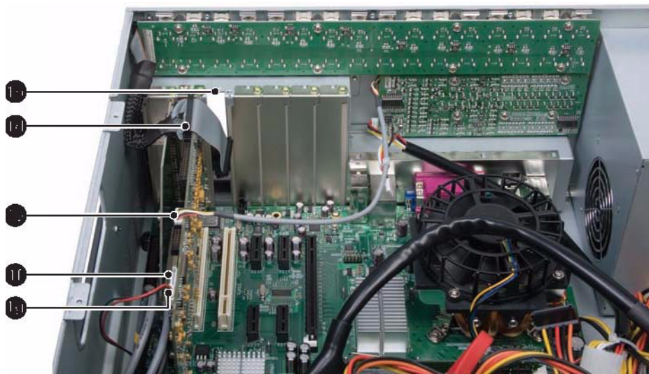
Figure 7. Readying Main Capture Card for Removal
