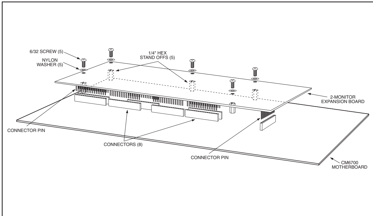
Figure 1. Exploded Assembly Diagram
