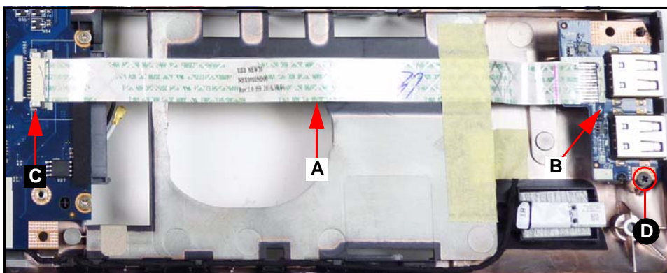
Figure 3-25. USB Module
