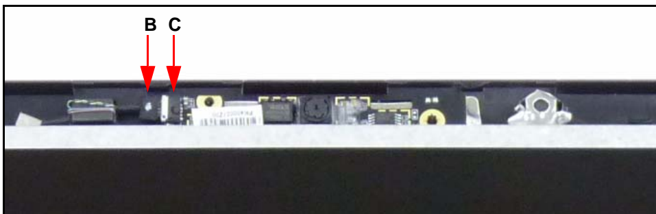
Figure 3-45. Camera Cable
