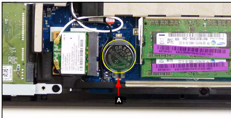
Figure 3-13. RTC Battery
