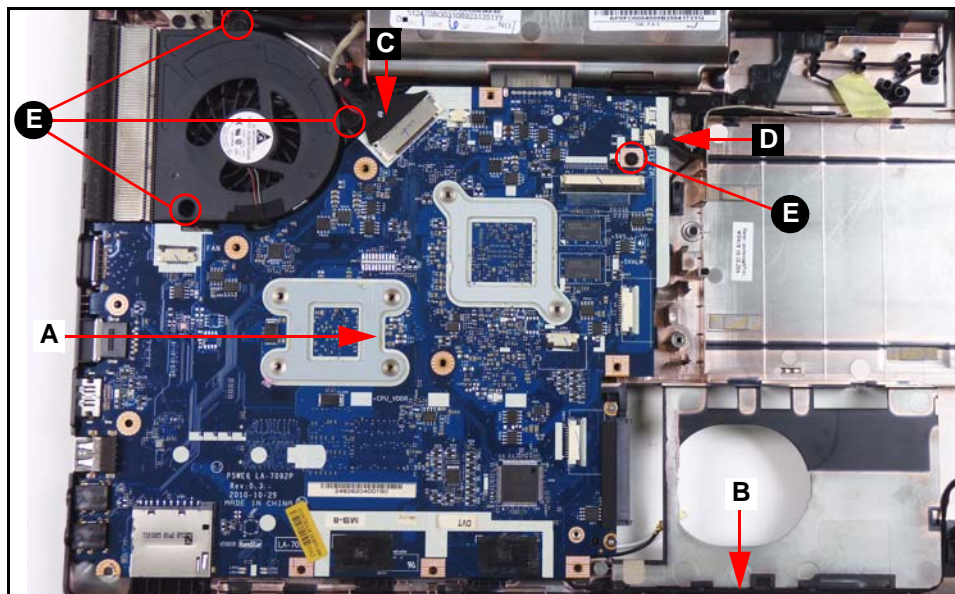
Figure 3-28. Mainboard Location
