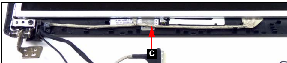
Figure 3-47. LVDS Cable
