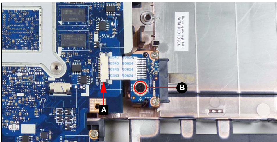
Figure 3-26. ODD Board
