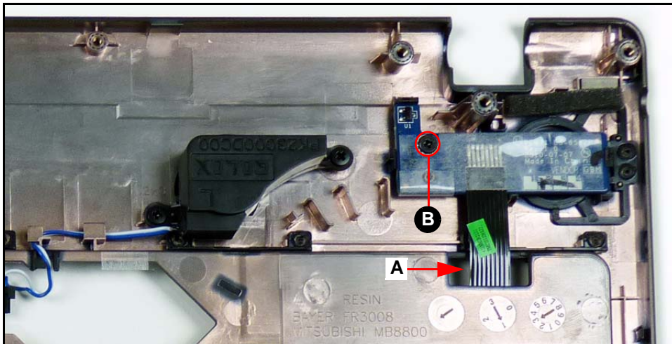
Figure 3-22. Power Board
