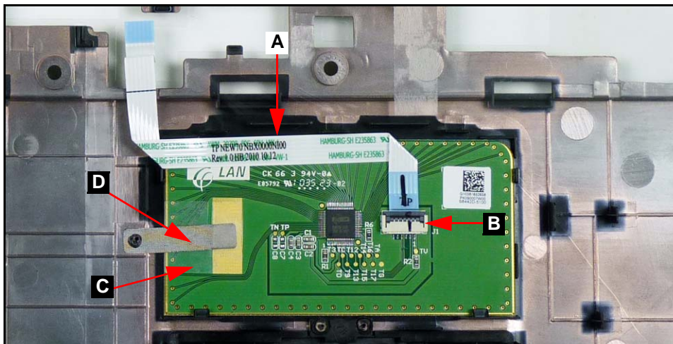
Figure 3-23. Touchpad
