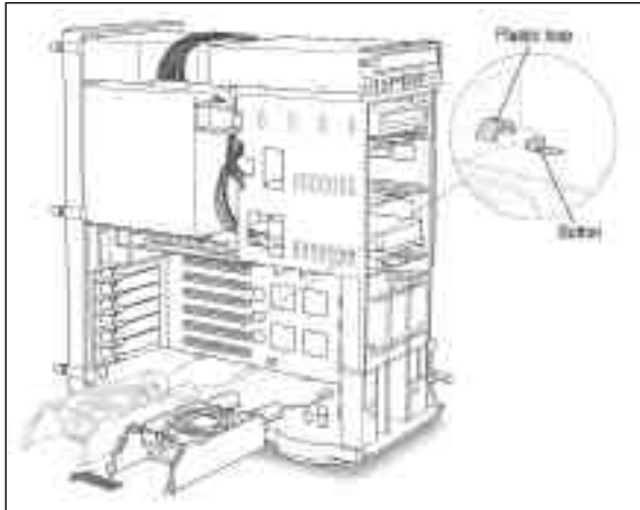
Reinstalling the fan (retaining clip on 8500)
