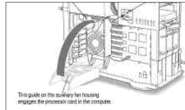
Lifting the auxiliary fan (retaining clip on 8500)
