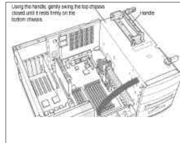
Swinging the chassis into place
