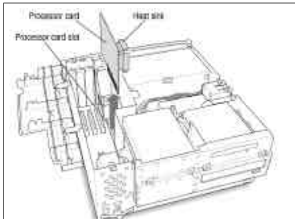
Removing the CPU card
