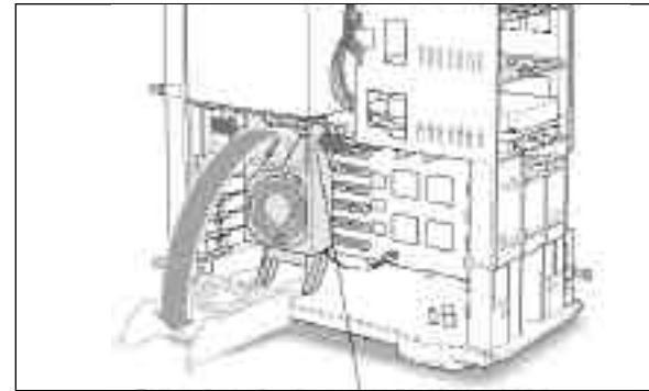
Lowering the auxiliary fan (retaining clip on 8500)
