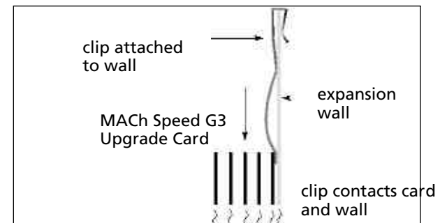
Cutaway view of the installed grounding clip
