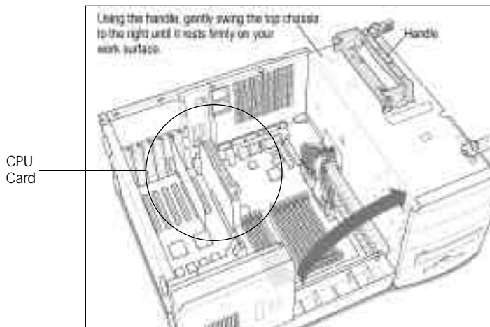
Swing the chassis to reveal the CPU card
