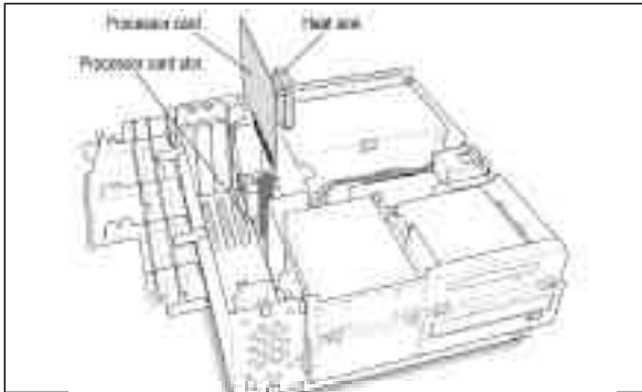
Removing the CPU card from a PowerMacintosh 7300
