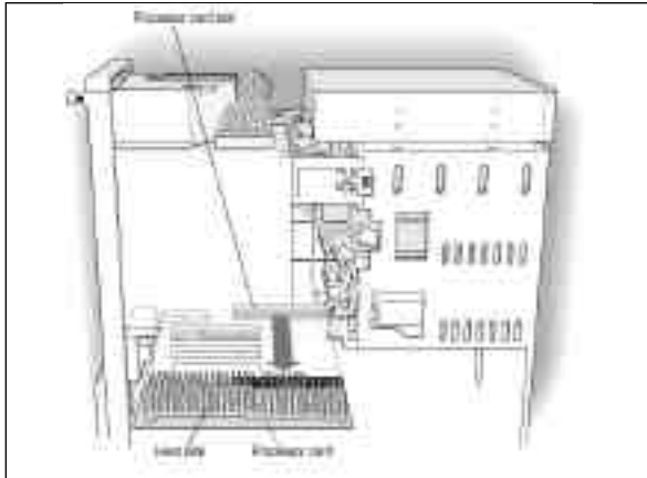
Removing the CPU card from a tower system
