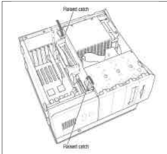
Rotating the locking levers
