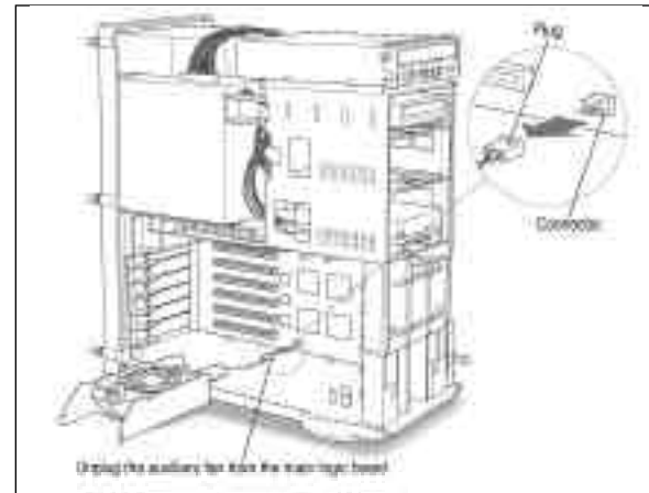
Unplugging the auxiliary fan (retaining clip on 8500)
