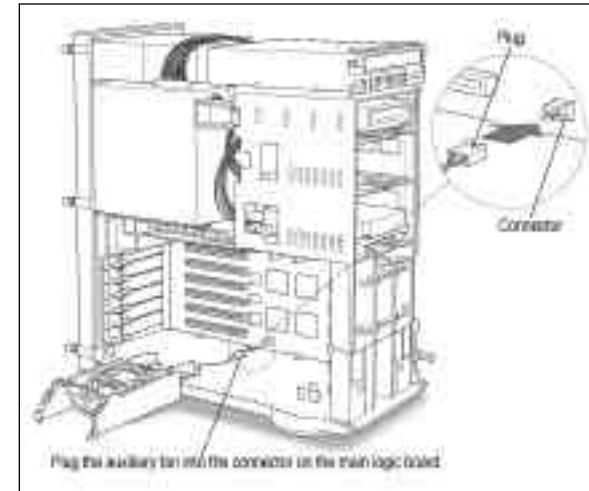
Attaching the fan power to the logic board
