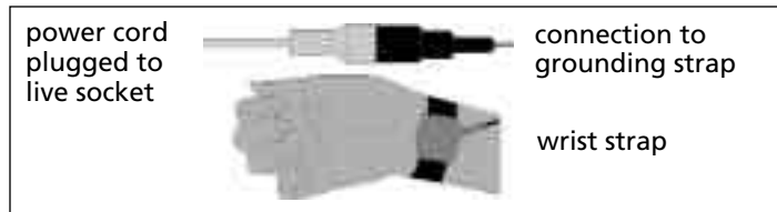
Attaching the anti-static wrist strap
