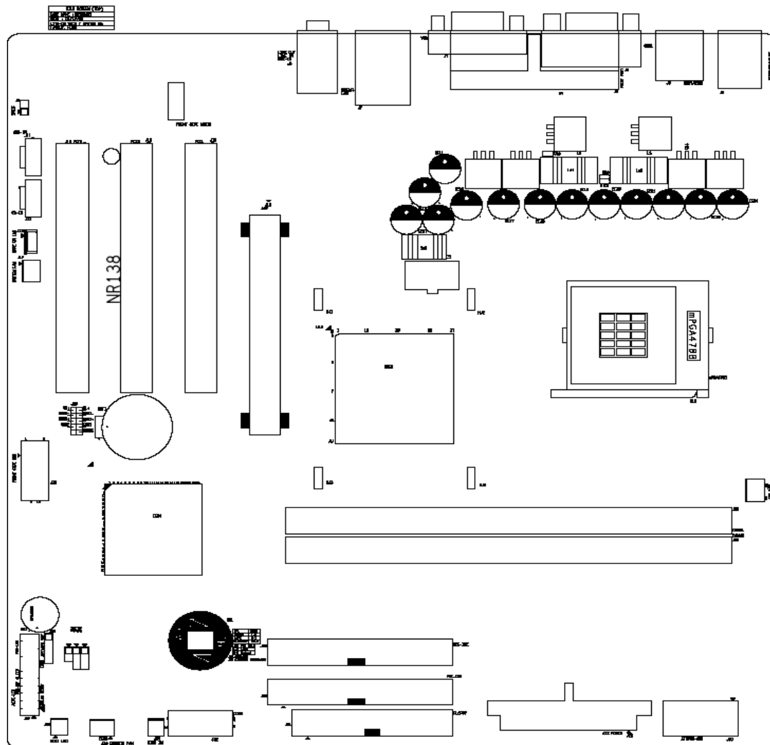
Figure 1-2. SCENIC Edition X101-Mainboard Layout Diagram
