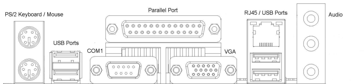
Figure 1-3. Back Panel Connectors
