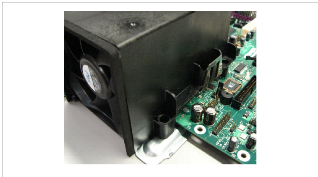
Figure 21. Heatsink Alignment
