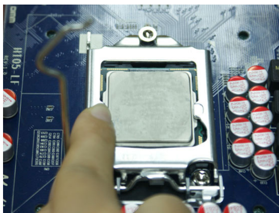
6. Put down the load plate in the direction shown above.
