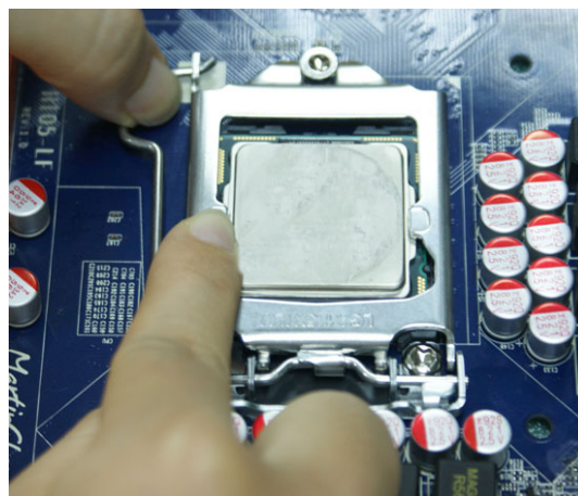
7. Press down the load level and move it rightwards make sure it is locked under the notch.
