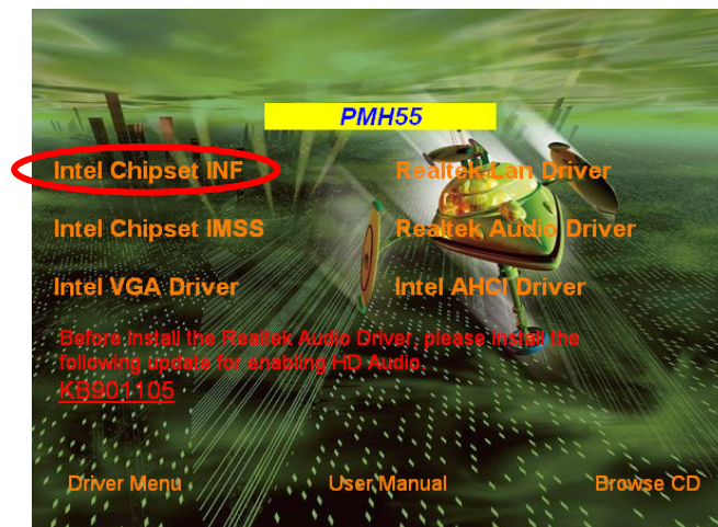
Windows XP 64
