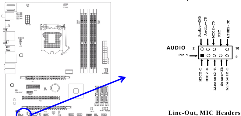
Line-Out, MIC Headers
