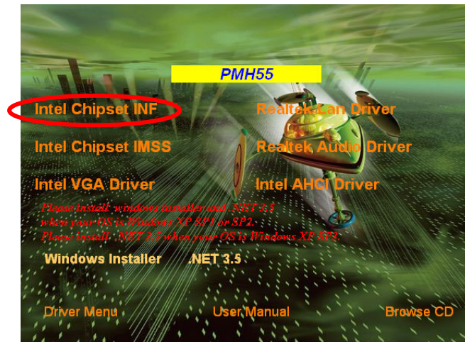
Windows XP
