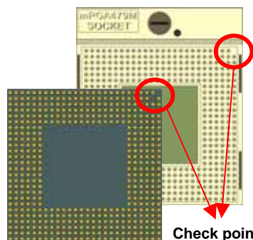
Embedded Intel Pentium M/Celeron M With 479-pin LV/ULV
