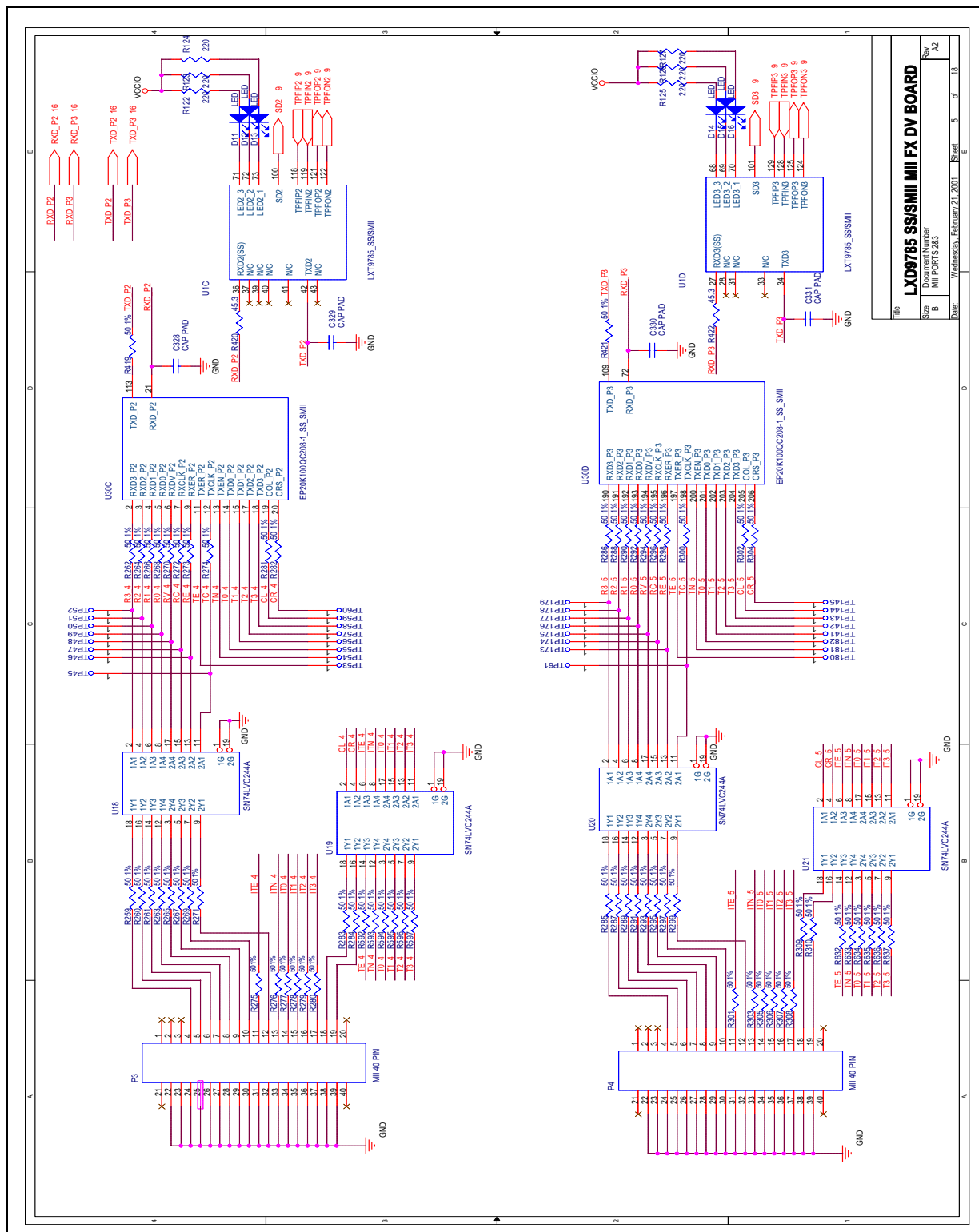
Figure 7. MII Ports 2 and 3
