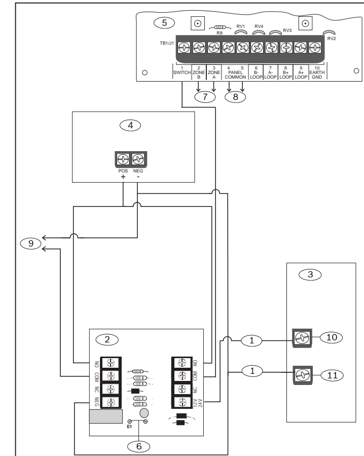
Figure 3.2: Wiring a D130 with 12 VDC or 24 VDC power supply and a D125B
